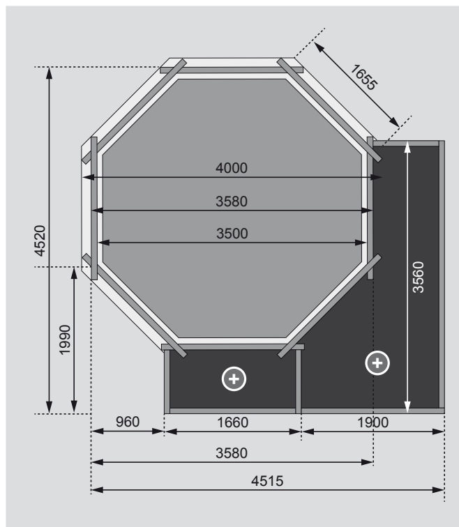
Fundament (in mm)
